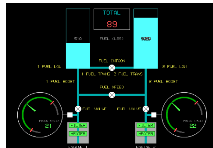
Example fuel system synoptic
