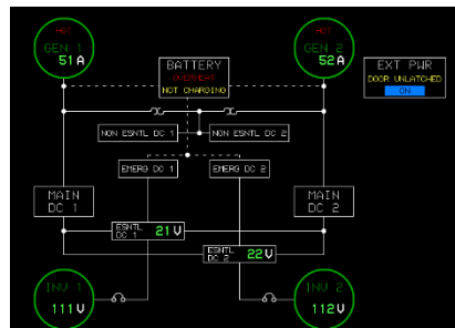
Example electrical system synoptic
